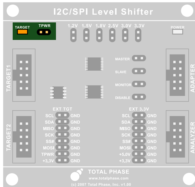
Figure 8: When supplying power from the Level Shifter Board to the target, a jumper needs to be placed on TPWR.
